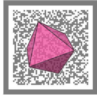
Octahedron
