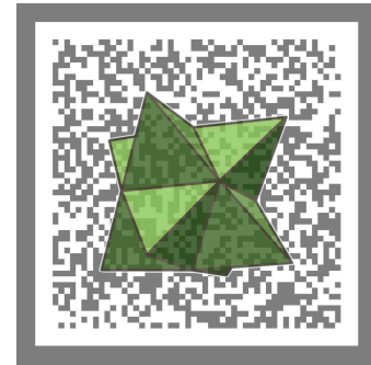
Dual Polyhedron 1
